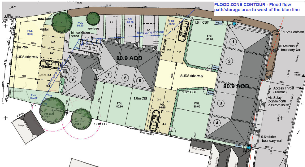
Extract from proposed layout plan
